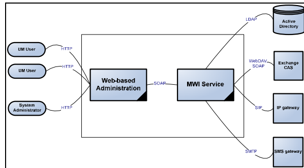
MWI2007 - Software architecture
