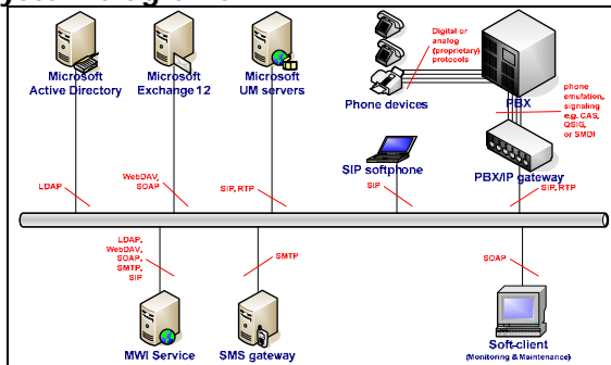
MWI2007 - System architecture
